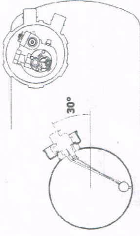
30° MONTAJI 30° INSTALLATION
